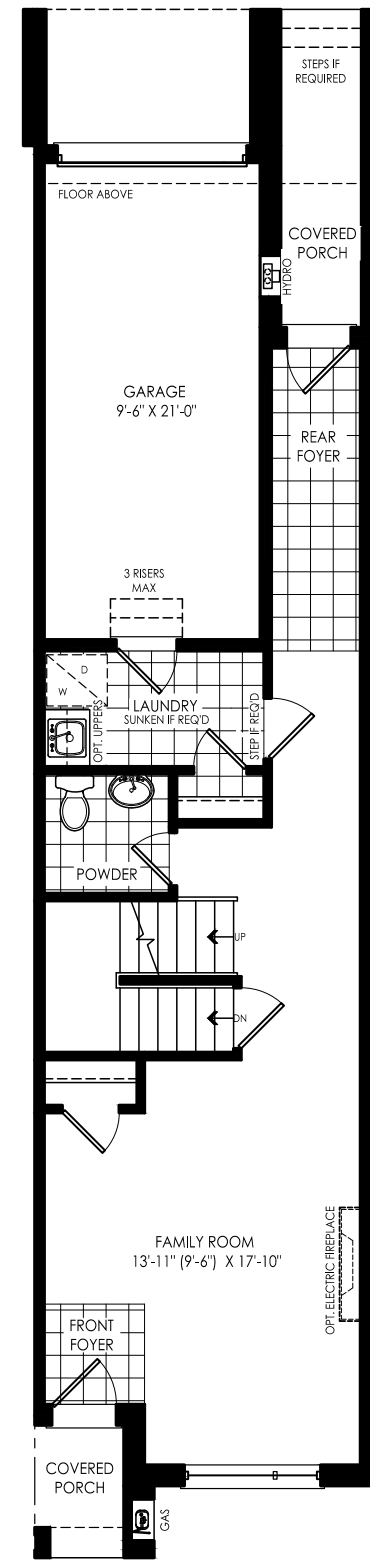
GROUND FLOOR PLAN ELEV. 'A'
