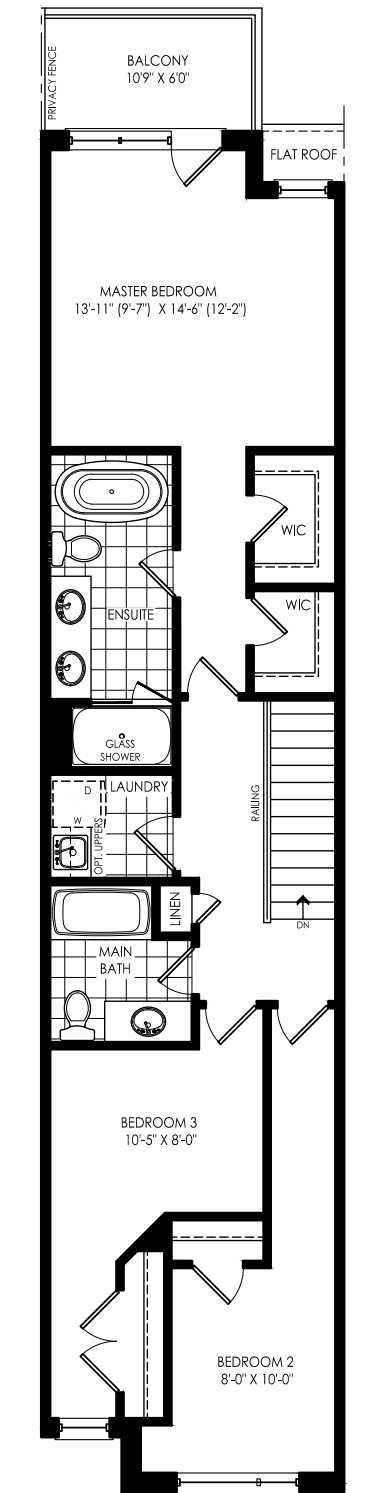
THIRD FLOOR PLAN ELEV. 'A'
