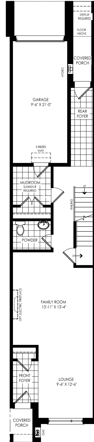
GROUND FLOOR PLAN ELEV. 'A'
