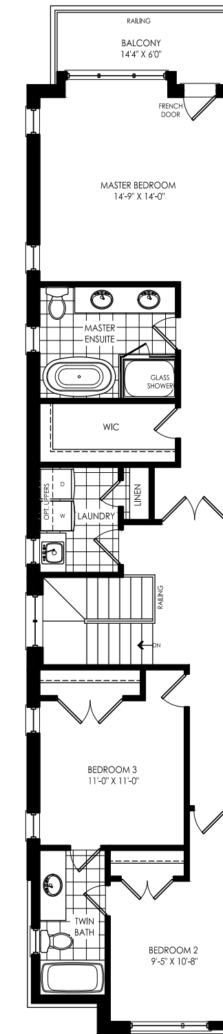
THIRD FLOOR PLAN ELEV. 'A'
