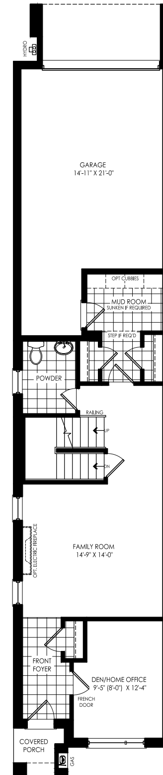
GROUND FLOOR PLAN ELEV. 'A'
