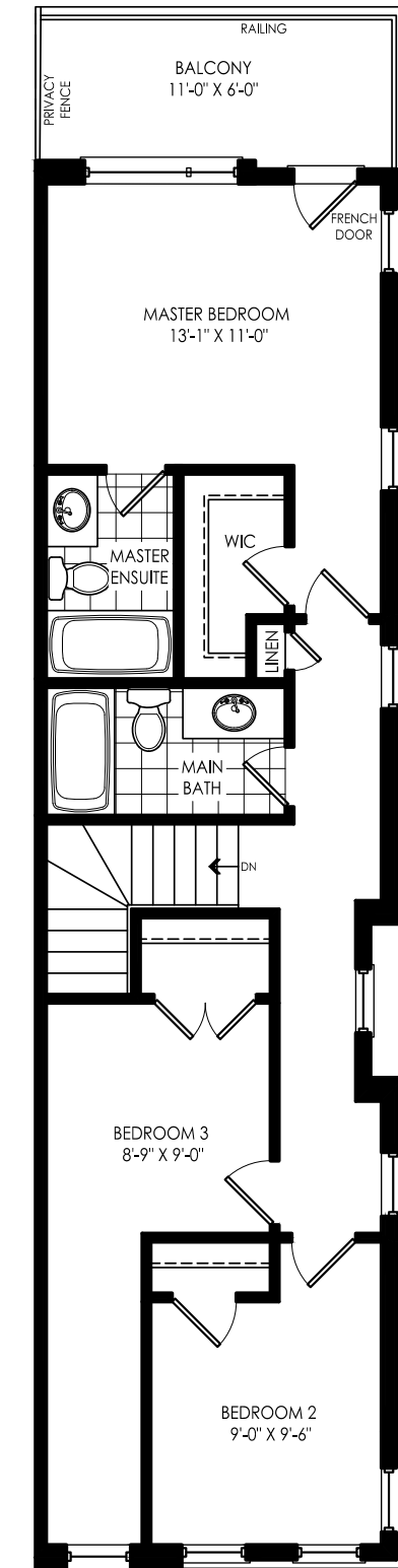
THIRD FLOOR PLAN ELEV. 'A'
