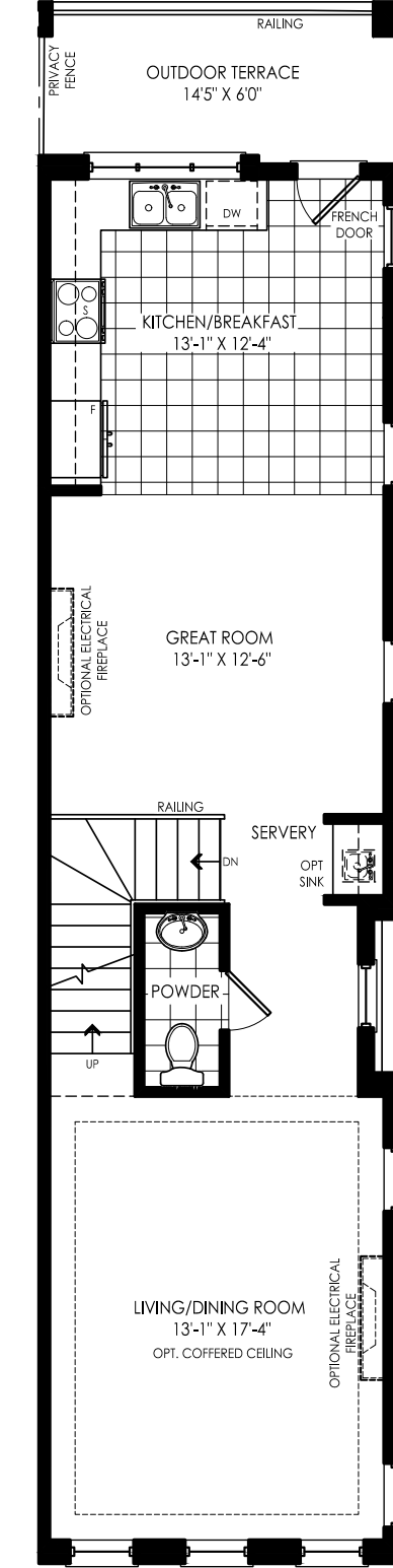
SECOND FLOOR PLAN ELEV. 'A'
