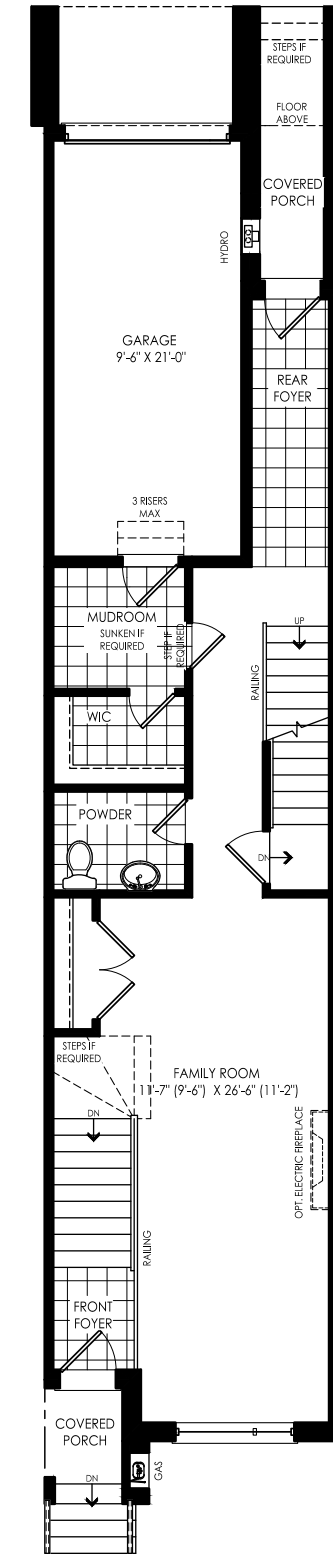
GROUND FLOOR PLAN ELEV. 'A'
