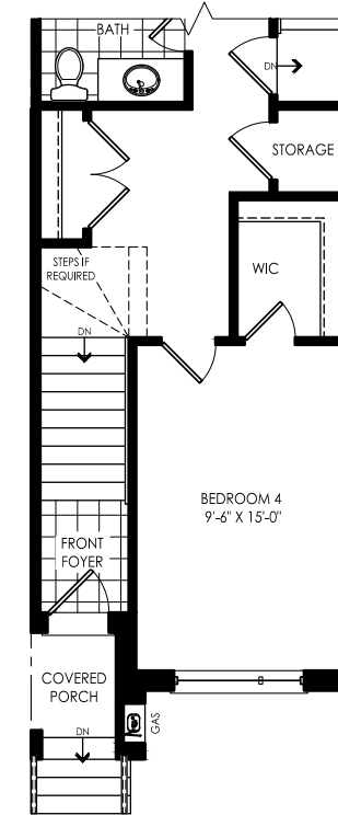
OPT. GROUND FLOOR PLAN ELEV. 'A'
