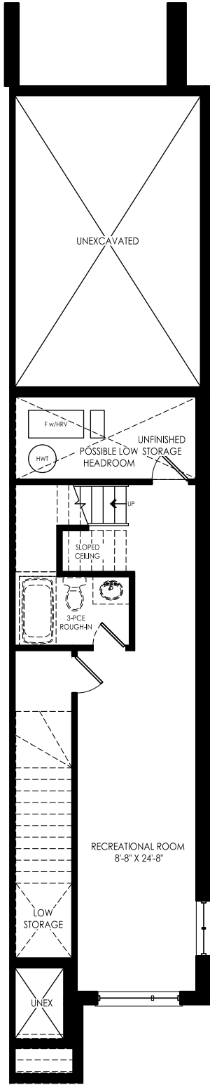
OPT. FINISHED BASEMENT PLAN ELEV. 'A' & 'B'
